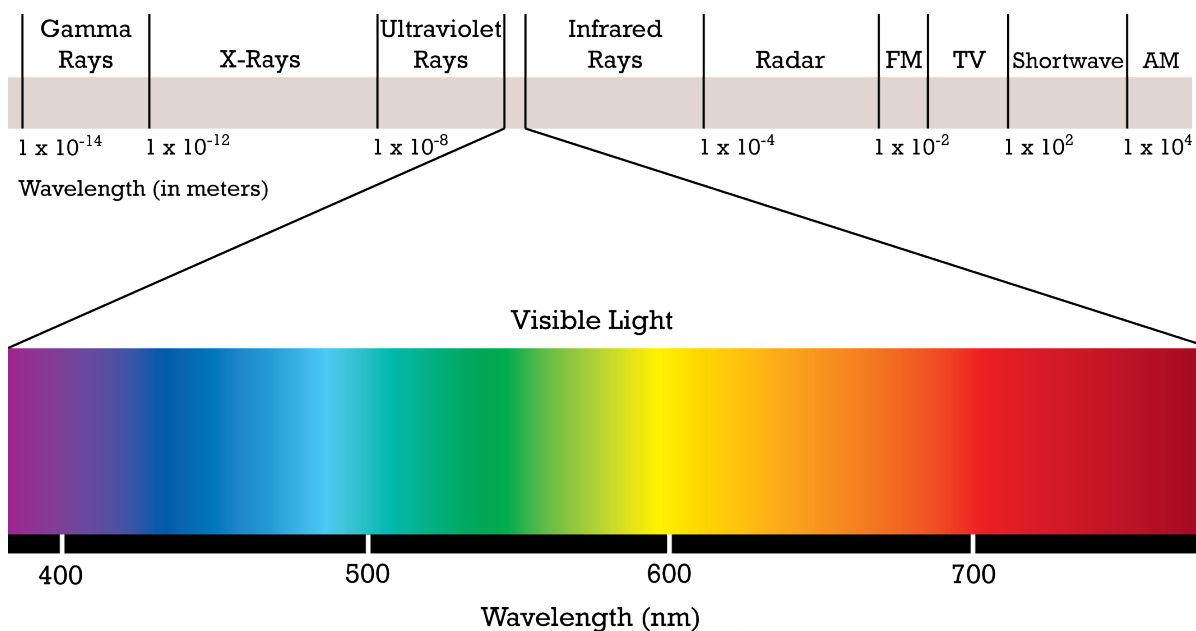
Figure 18. Electromagnetic spectrum.
